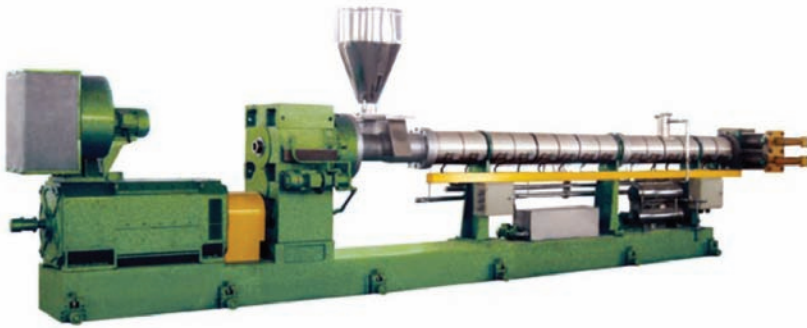
SJ 160mm Single Screw Extruder 36:1 L/D
