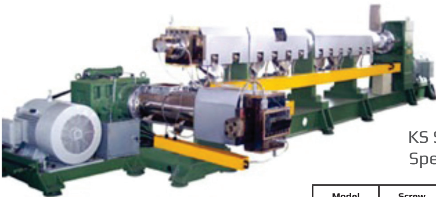
KS150/170 two-stage Recycling Extrusion Line
